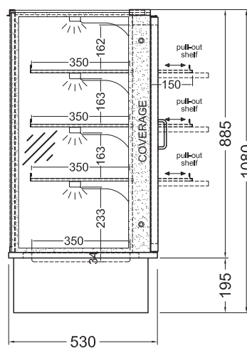
(side elevation)
